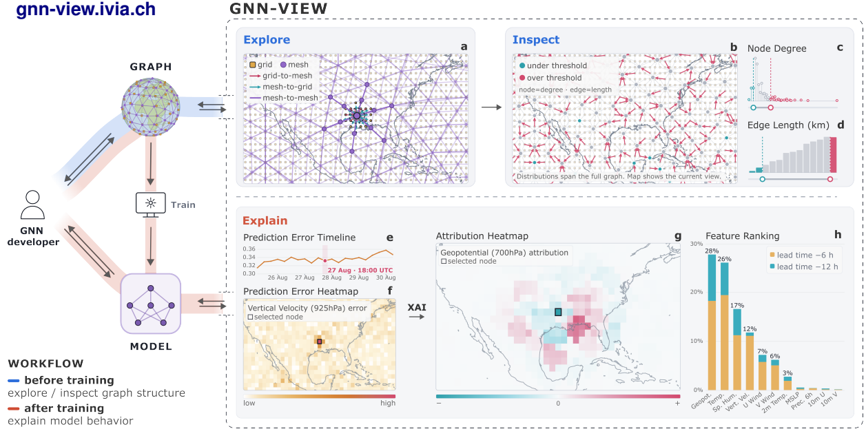
Fig. 1: GNN-VIEW lets developers explore graph structure (a–d) and explain prediction errors with attribution-based explanation (e–h).
