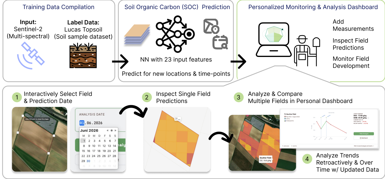
Fig. 1: The AgroScan Workflow: Schematic overview of the AgroScan web-tool showing the user interaction workflow. The workflow is enabled by an SOC prediction pipeline based on training data compiled from satellite imagery and the LUCAS soil dataset. By predicting SOC for novel locations and time-points, farmers can analyze values for individual selected fields for any time-point satellite images are available. We support the user workflow with a personalized monitoring and analysis dashboard enabling comparative analysis, as well as temporal trend analysis.
